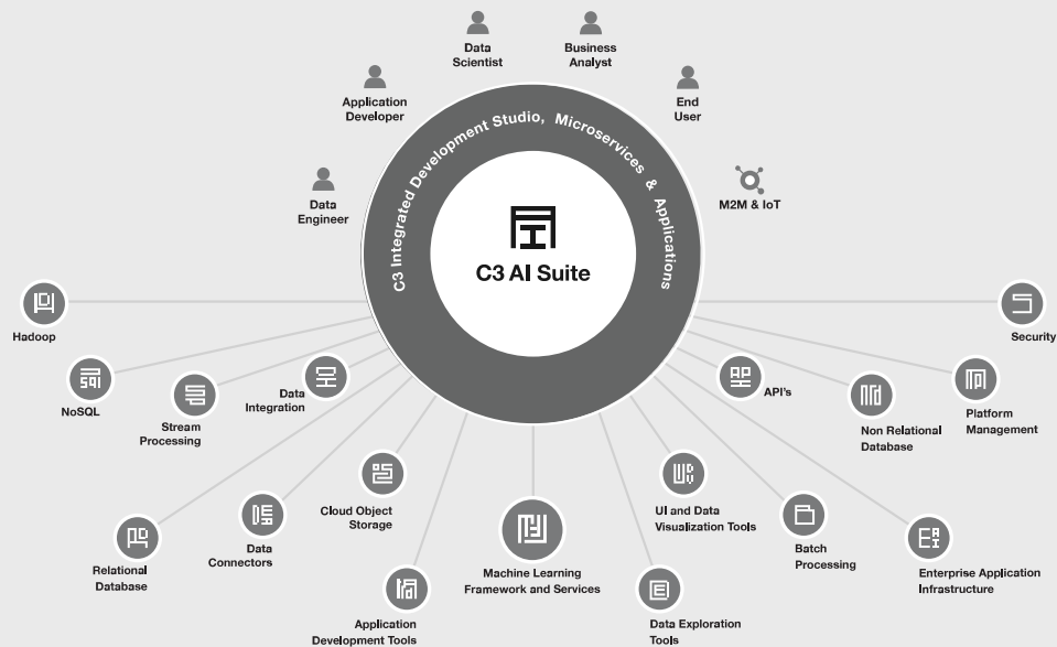
Figure: Model-Driven Architecture Abstracts Underlying Platform Services through a simple Type Systems Interface
